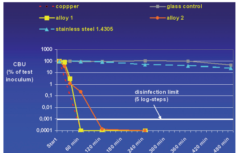
Fig 1: Results on the test JIS Z 2801 [8] with copper, Cu-alloys and stainless steel coupons. The inoculum (Staphylococcus aureus ATCC 6538) was about 1.000.000 cfu (colony forming units) per coupon (50 * 50 mm) each. A reduction rate of > 5 log steps is needed for disinfection.
